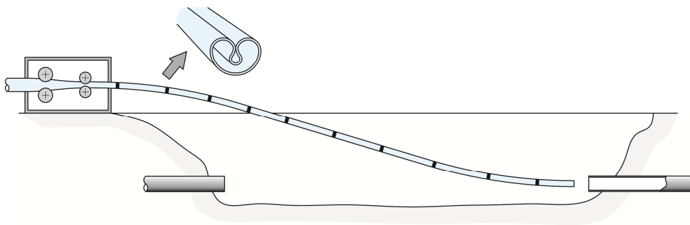
Fig. 14 - U-lining
