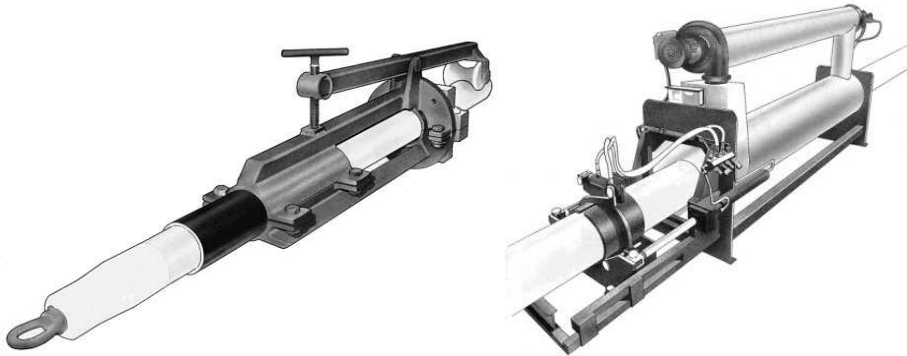
Fig. 13 - Swagelining
