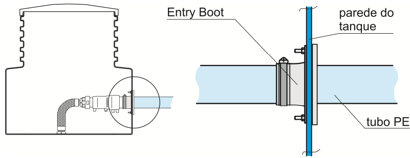
Fig.15- Entry boot de borracha
